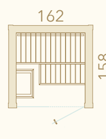
MIRA S in natural cladding
